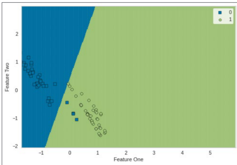
Figure 3: Decision Boundary
