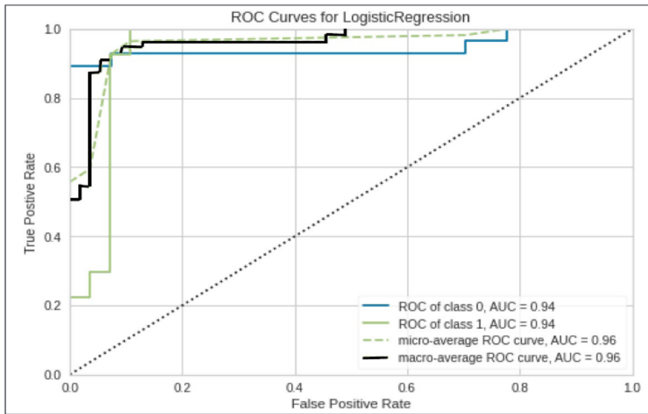
Figure 2 – ROC Curve
